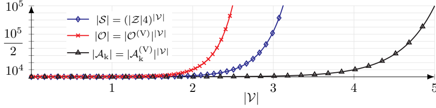
Figure 3.2: Growth of |\mathcal{S}| , |\mathcal{O}| , and |\mathcal{A}_k| in function of the number of nodes |\mathcal{V}| ; the curves are computed using |\mathcal{Z}| = 10 , |\mathcal{O}^{(V)}| = 100 , and |\mathcal{A}_D^{(V)}| = |\mathcal{A}_A^{(V)}| = 10 .
