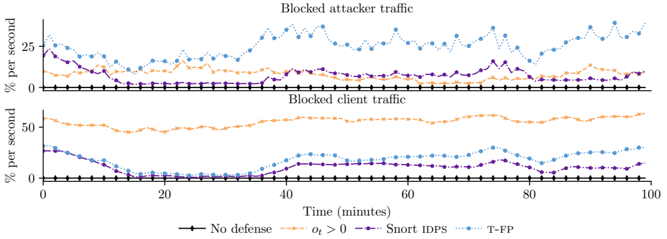
Figure 2.10: Percentage of blocked attacker and client traffic in the digital twin ; the blue curves show results from the equilibrial strategy learned via T-FP ; the purple, orange, and black curves relate to baseline strategies.
