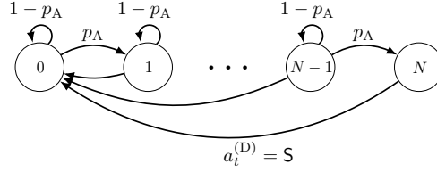
Figure 5.2: State transition diagram of the game \Gamma : disks represent states; arrows represent transitions; labels indicate conditions for transition; the initial state is s_1 = 0 .
