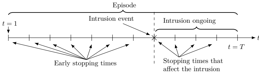
Figure 1.1: Optimal multiple-stopping formulation of intrusion prevention; the horizontal axis represents time; T is the time horizon; the dashed line shows the intrusion start time; the optimal strategy is to prevent the attacker at the time of intrusion.
