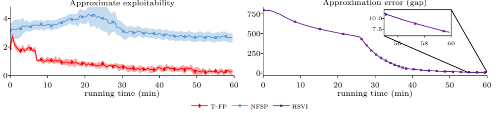
Figure 2.8: Comparison between T-FP and two baseline algorithms: NFSP and HSVI; all curves show simulation results; the red curve relates to T-FP; the blue curve to NFSP; the purple curve to HSVI; the left plot shows the approximate exploitability metric (2.13) and the right plot shows the HSVI approximation error; the curves depicting T-FP and NFSP show the mean and the 95% confidence interval over four random seeds.
