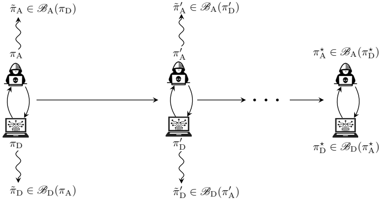
Figure 27: The fictitious play process between the attacker and the defender in Paper 2 ; horizontal arrows indicate iterations of fictitious play and vertical arrows indicate the learning of best responses; the process converges to an equilibrium (\pi_D^*, \pi_A^*) .
