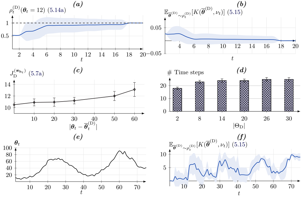
Figure 5.13: Evaluation results for Scenario 5.2; values indicate the mean; the shaded areas and the error bars indicate the 95% confidence interval based on 20 random seeds; hyperparameters are listed in Appendix F.
