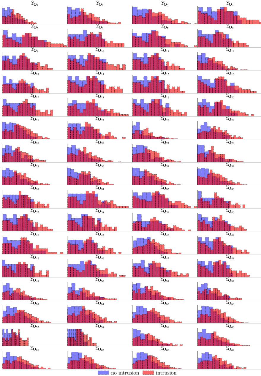
Figure 3.7: Empirical observation distributions \hat{z}_{\mathbf{O}_1}, \dots, \hat{z}_{\mathbf{O}_{|\mathcal{V}|}} as estimates of z_{\mathbf{O}_1}, \dots, z_{\mathbf{O}_{|\mathcal{V}|}} in the target infrastructure; \mathbf{O}_i is a random variable representing the number of IDS alerts related to node i \in \mathcal{V} , weighted by priority; the x-axes show the node-local observation spaces \mathcal{O}^{(\mathcal{V})} ; the y-axes show \hat{z}_{\mathbf{O}_i}(\mathbf{o}_i | \mathbf{s}_i) (3.3).
