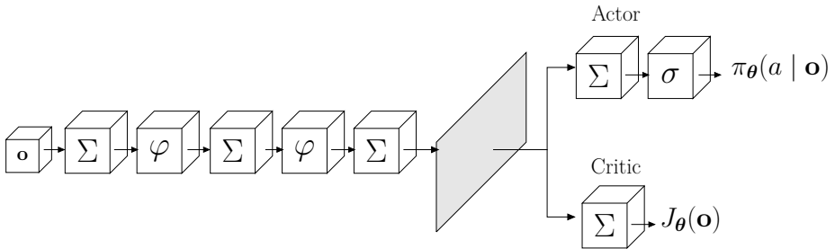
Figure 1.9: Architecture of the neural network used by PPO ( Alg. 1, Schulman et al., 2017 ); the strategy \pi_{\theta} and the value function J_{\theta} are parameterized by a neural network with the actor-critic architecture ( Sutton and Barto, 1998 ); \Sigma represents a linear sum; \sigma represents the softmax function; and \varphi represents the RELU function.
