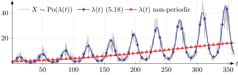
Figure 5.10: The arrival rate function (5.18) used in Scenario 5.2 ; the blue curve shows the arrival rate \lambda(t) ; the red curve shows the trend of \lambda(t) without the periodic effects; and the shaded black curve shows the number of arrivals.
