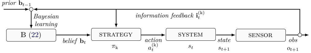
Figure 17: The control loop of player k in a partially observed stochastic game (19).
