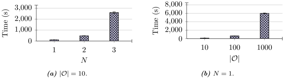
Figure 5.6: Time required to compute a Perfect Bayesian equilibrium (PBE) of \Gamma (5.1) with HSVI (Alg. 1, Horák et al., 2017) for different values of N (Fig. 5.6.a) and |\mathcal{O}| (Fig. 5.6.b); error bars indicate the 95% confidence interval based on 20 measurements; hyperparameters are listed in Appendix F.
