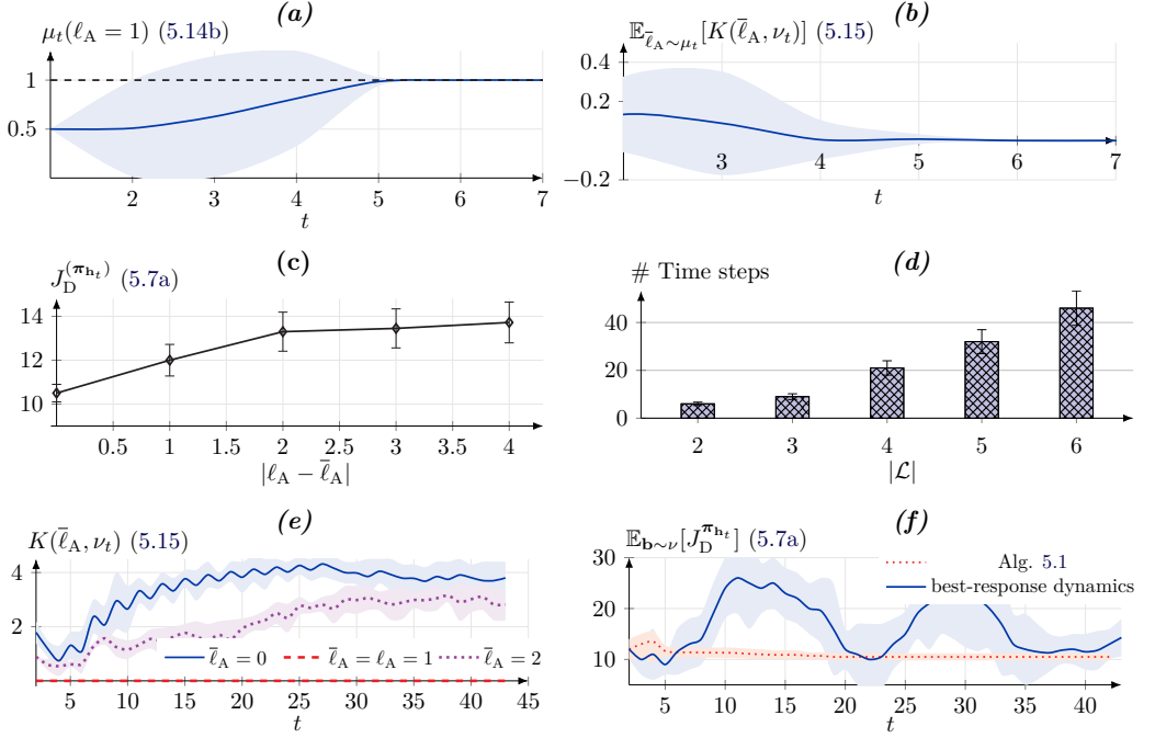
Figure 5.12: Evaluation results for Scenario 5.1 ; values indicate the mean; the shaded areas and the error bars indicate the 95% confidence interval based on 20 random seeds; hyperparameters are listed in Appendix F .
