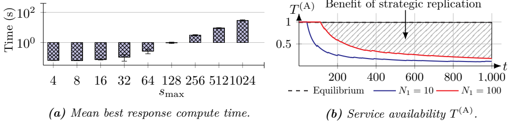
Figure 4.12: Plot a) shows the compute time to obtain a best response in Game 4.2 via the linear program in Alg. 4.2 ; the error bars indicate the 95% confidence interval based on 20 runs; s_{\max} is the maximum number of nodes; plot b) shows the availability of the equilibrium strategy and two fixed replication strategies with different number of nodes N_1 ; hyperparameters are listed in Appendix G .
