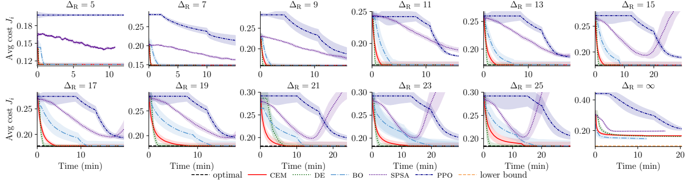
Figure 4.8: Convergence curves of Alg. 4.1 for computing a best response control strategy in Game 4.1 (the local intrusion recovery game); the curves relate to different parametric optimizers: SPSA, BO, CEM, DE, and PPO; the curves show the mean value from evaluations with 20 random seeds and the shaded areas indicate the 95% confidence interval divided by 10.
