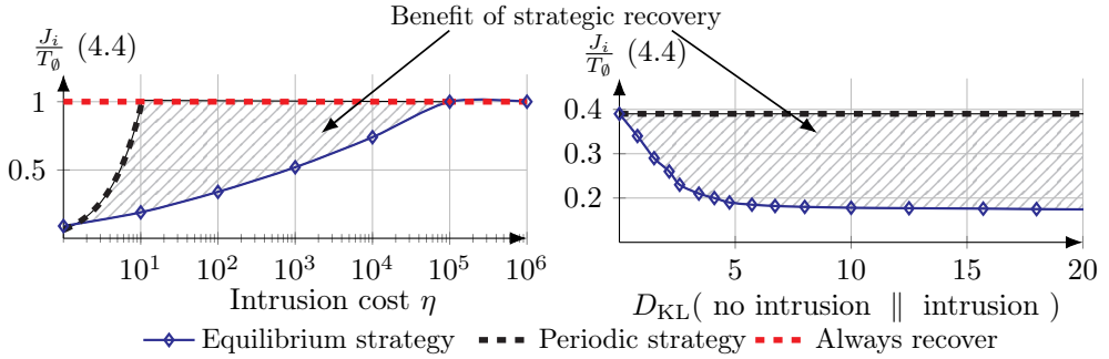
Figure 4.9: Comparison between the operational cost incurred by equilibrium and periodic strategies in Game 4.1 as functions of \eta (4.4) and the KL divergence between z_i(\cdot | F) and z_i(\cdot | A) (4.2); hyperparameters are listed in Appendix G; the values were computed using the HSVI algorithm (Alg. 3, Horák et al., 2023); when computing the value of the periodic strategy, we restricted the strategy space of the controller to the class of periodic strategies.
