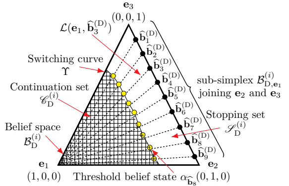
Figure 3.5: Theorem 3.2.C.
